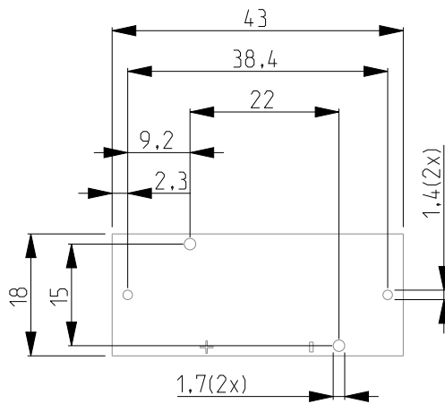
Layout on printed circuit board TOP VIEW
